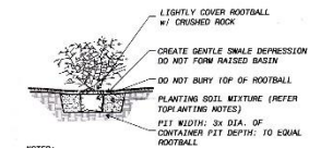
3 Shrub Planting NTS
