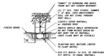
1 Typical Foundation & Island Planting 1" = 20'
